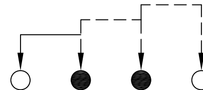
SCHEMATIC (NON-SHORTING)
